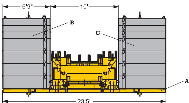
CWT at superstructure Contrepoids tourelle
